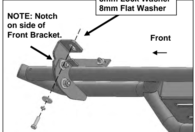
(Fig 11) Passenger/right side Front Bracket illustrated for vehicles with threaded inserts
