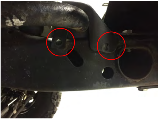
Step 1\\ Remove the push clips holding the bumper trim panel.
