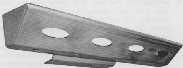
17-59-030 JK Brawler Lite Front Skid Plate
