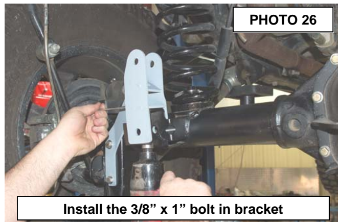
Position the bracket and install hardware
