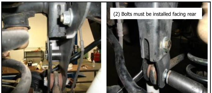
26. Install rear track bar extension bracket with provided hardware and spacers.
