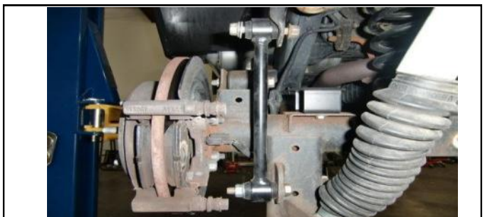
28. Install rear 11" sway bar end links with supplied hardware.
