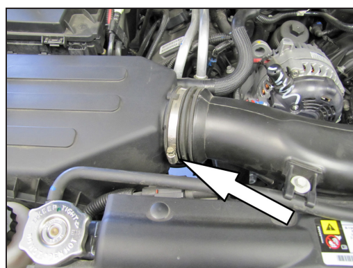
4. Loosen the hose clamp securing the factory intake tube to the air filter housing.
