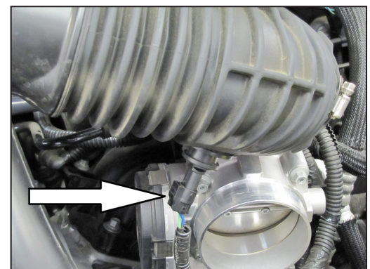
6. Lift up the intake tube, disconnect the inlet air temperature electrical connection then remove the intake tube from the vehicle.
