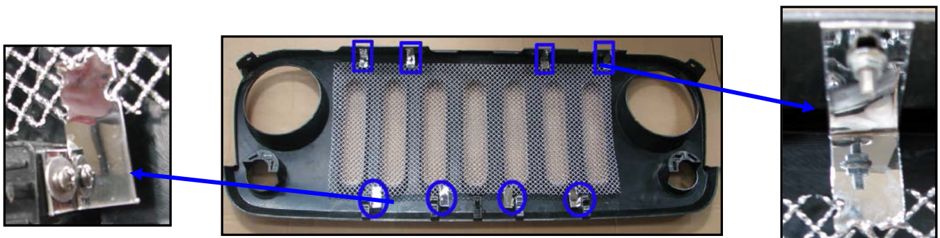
Figure 3 – Rear view of vehicle's shell; Grills attached with Metal Brackets and Flange Nuts
